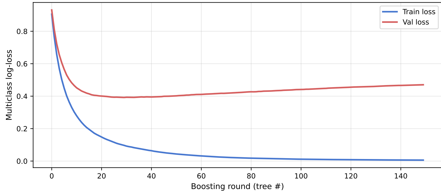
XGBoost Training Curve (3k train + 1.5k val, mini demo)
