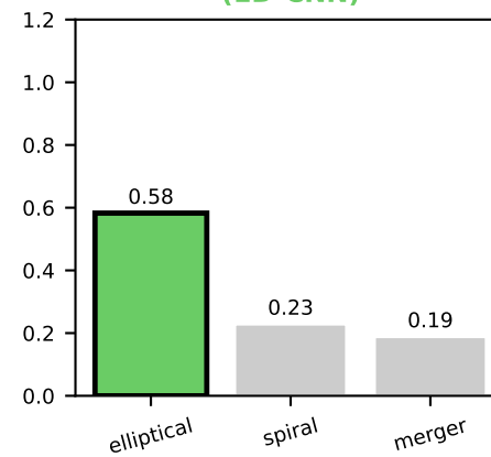
Spectral (1D-CNN)
