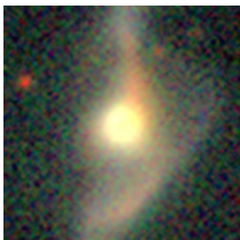
True: merger
