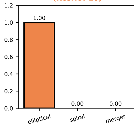
Image (ResNet-18)
