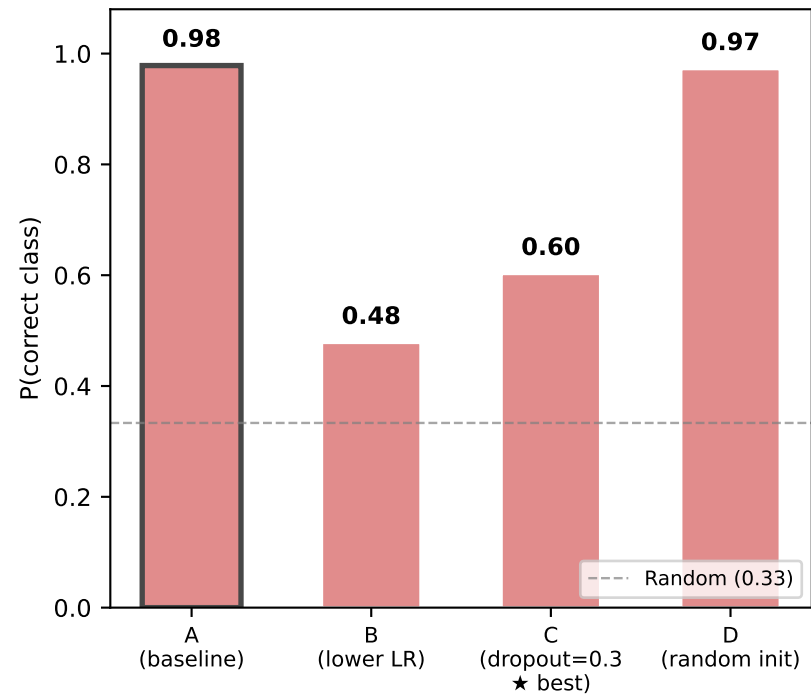
Merger sample
