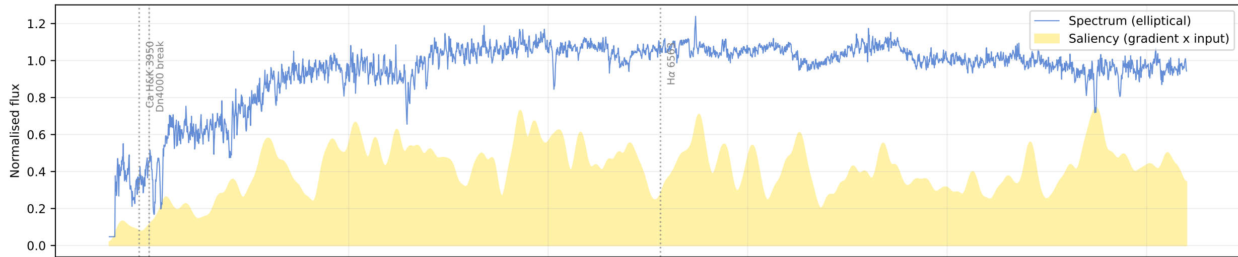
Elliptical galaxy — regions the 1D-CNN attends to
