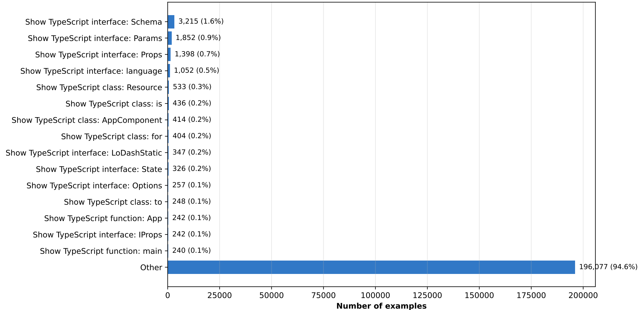
expert-typescript dataset: top sections
