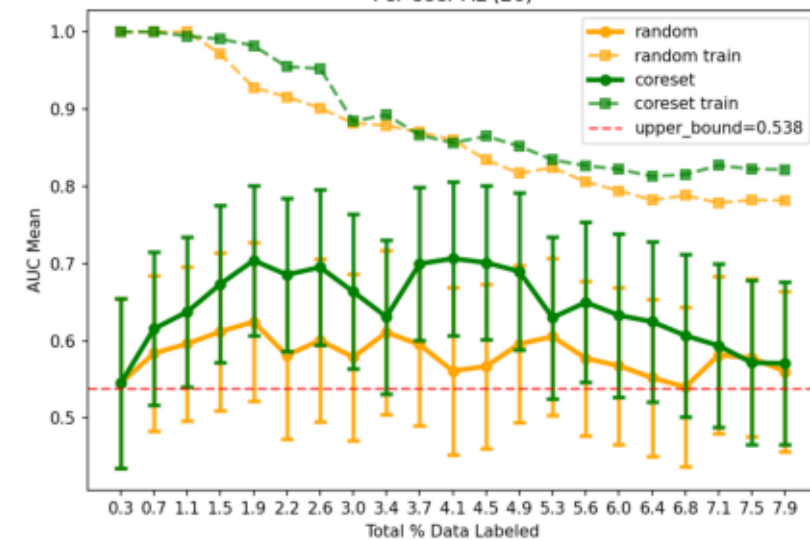
Per-User AL (26)
