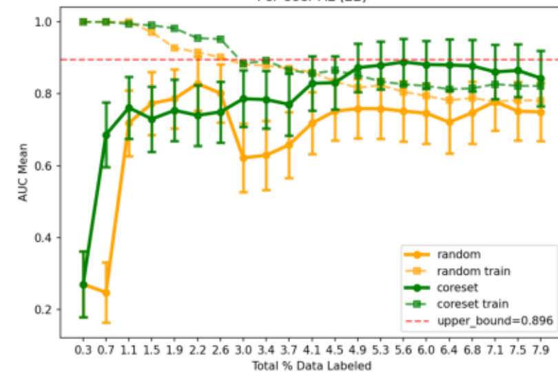
Per-User AL (22)
