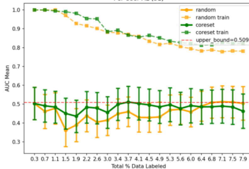
Per-User AL (31)
