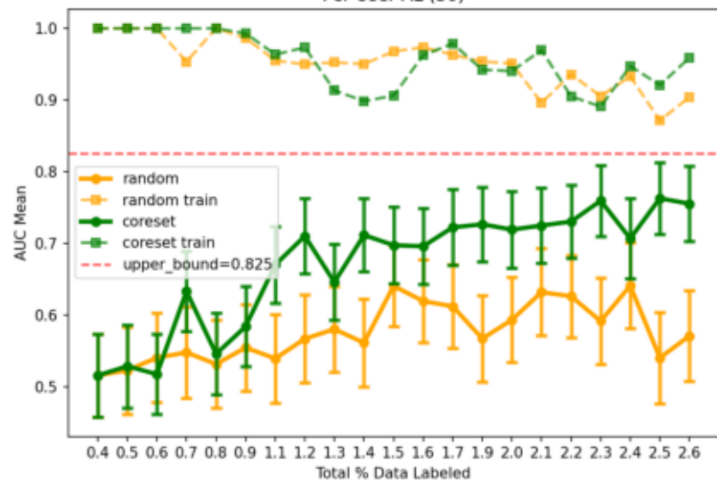
Per-User AL (30)
