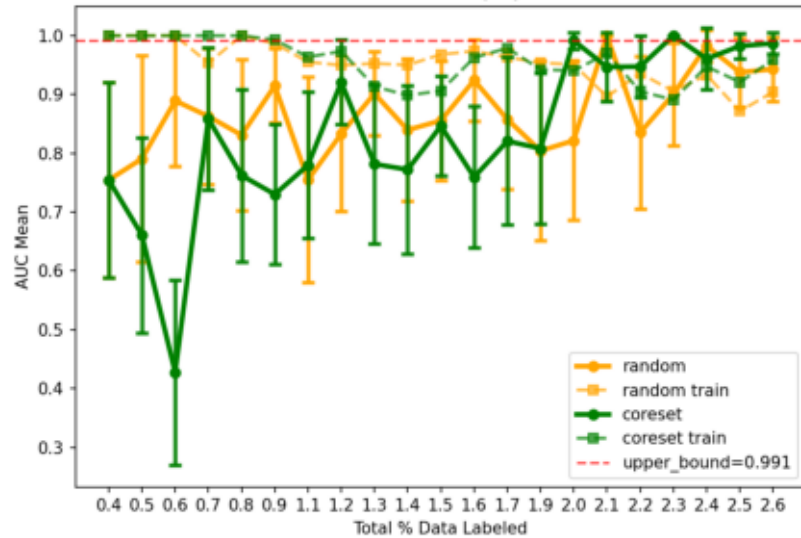
Per-User AL (39)
