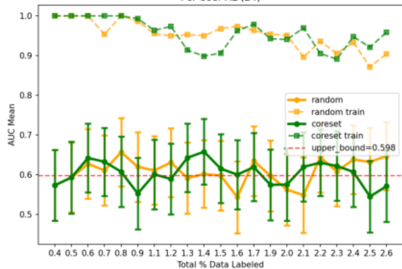
Per-User AL (24)
