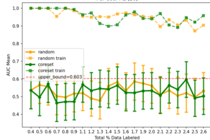
Per-User AL (26)
