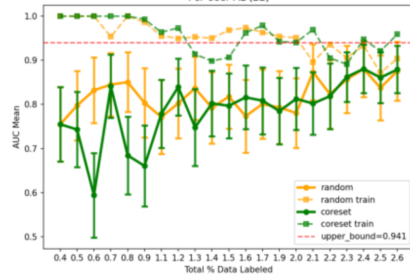
Per-User AL (22)
