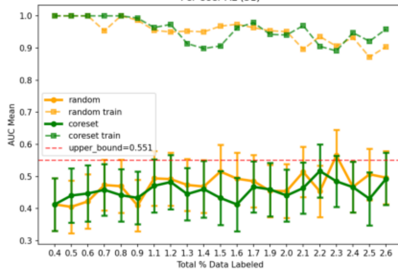
Per-User AL (31)
