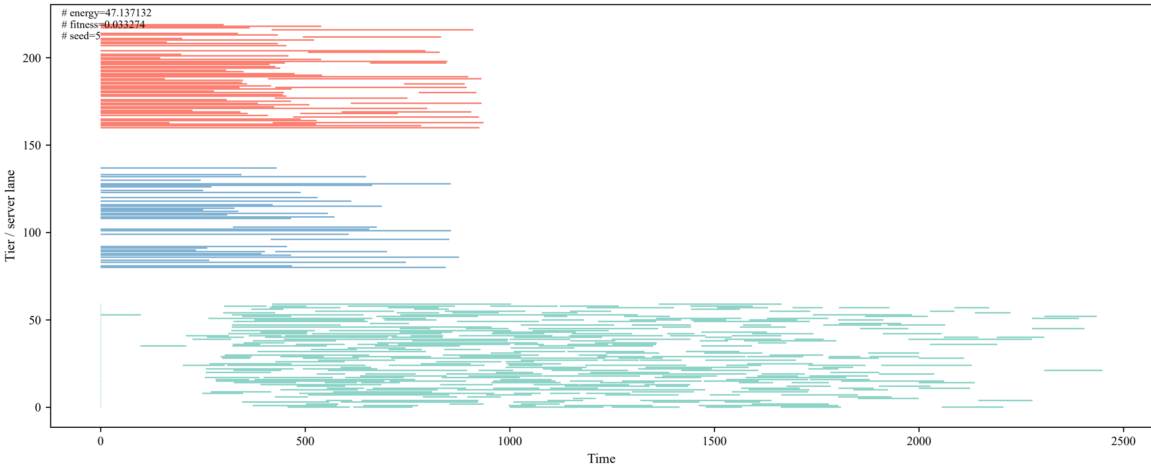
Gantt chart for T200 best schedule
