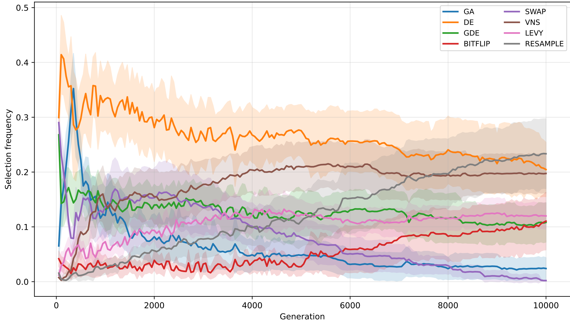
T100 Bandit Operator Frequency (overall, mean \pm 95% CI)
