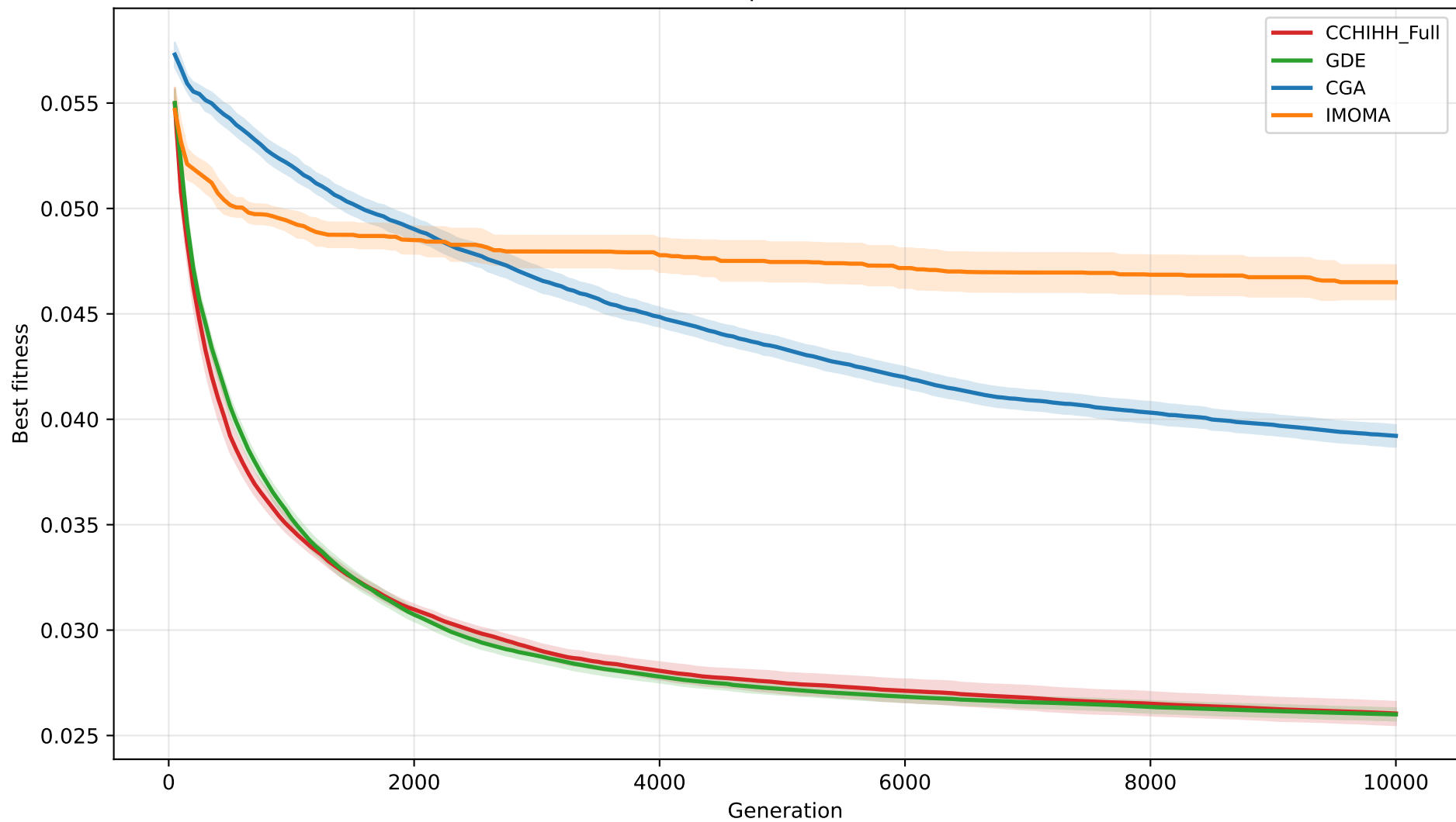
T500 Baseline Comparison (mean \pm 95% CI)
