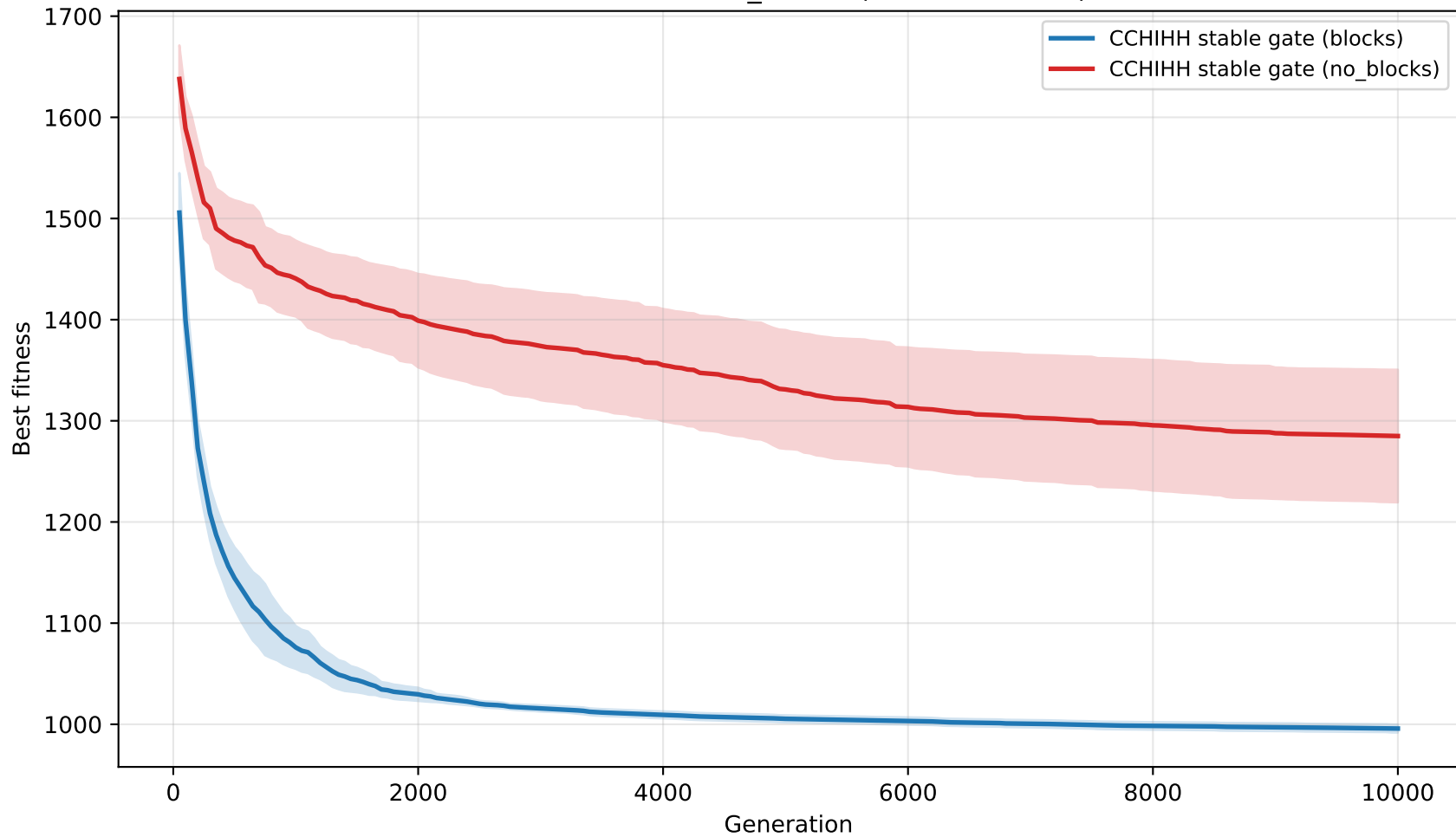
T200: blocks vs no_blocks (mean \pm 95% CI)
