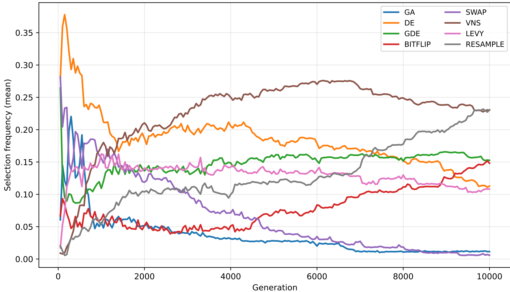
CCHIIH cfg1 Operator Frequency - overall (mean)
