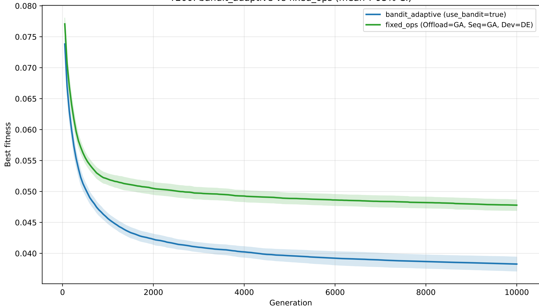
T200: bandit_adaptive vs fixed_ops (mean ? 95% CI)
