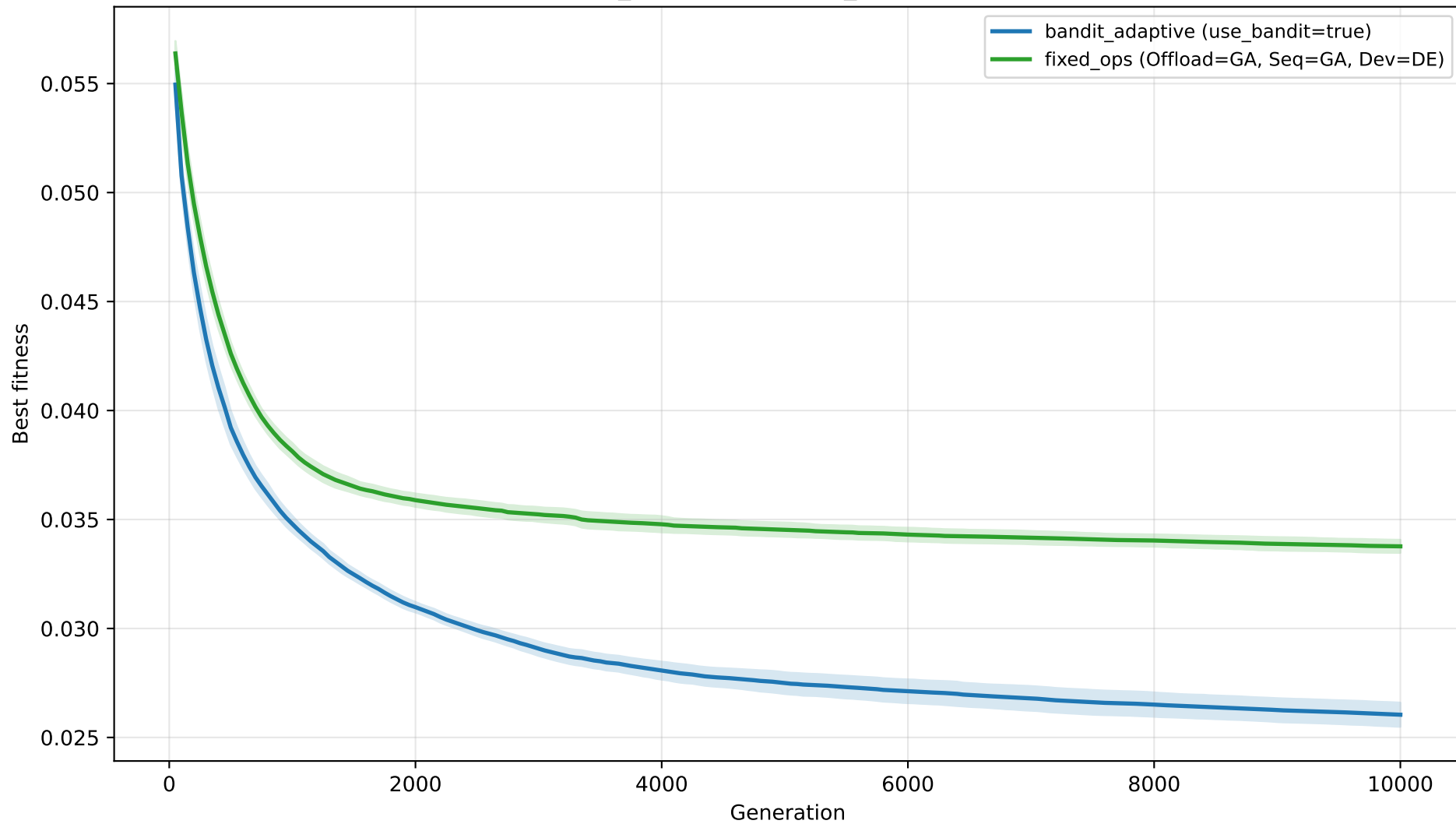
T500: bandit_adaptive vs fixed_ops (mean ? 95% CI)
