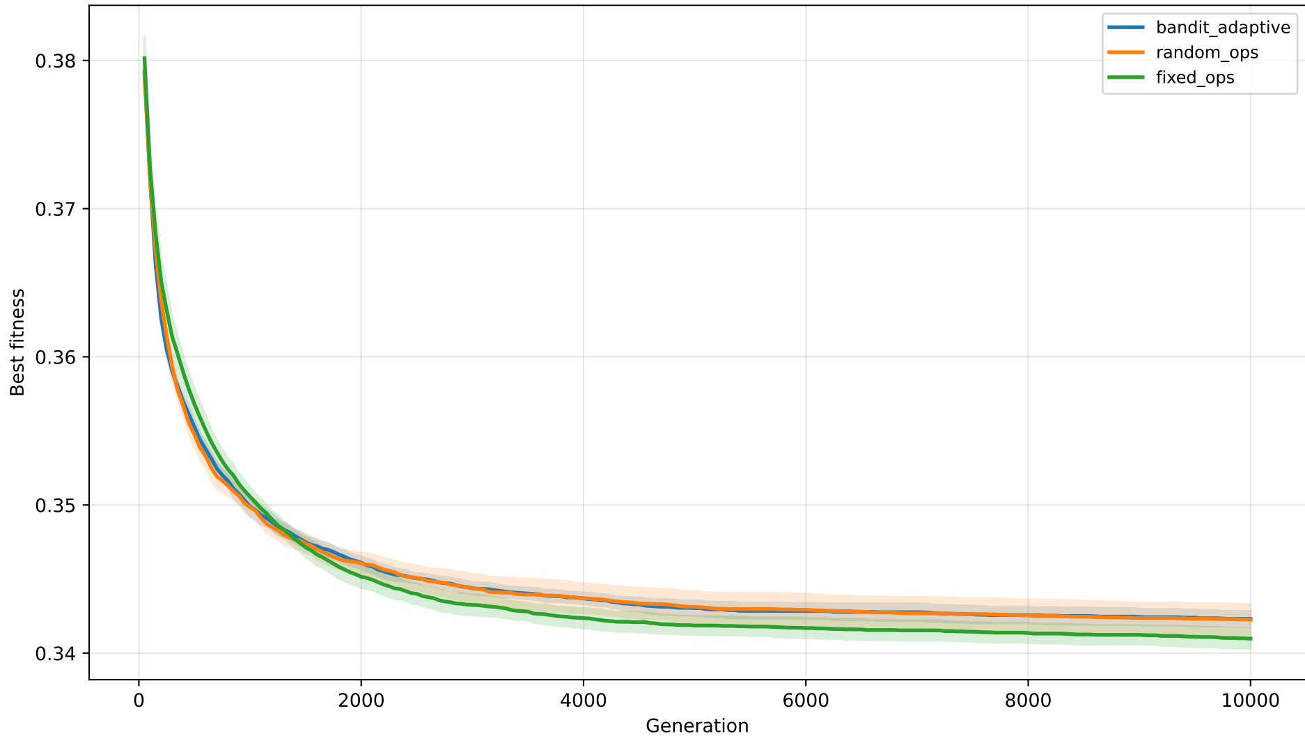
T100 Contextual Bandit Ablation (mean \pm 95% CI)
