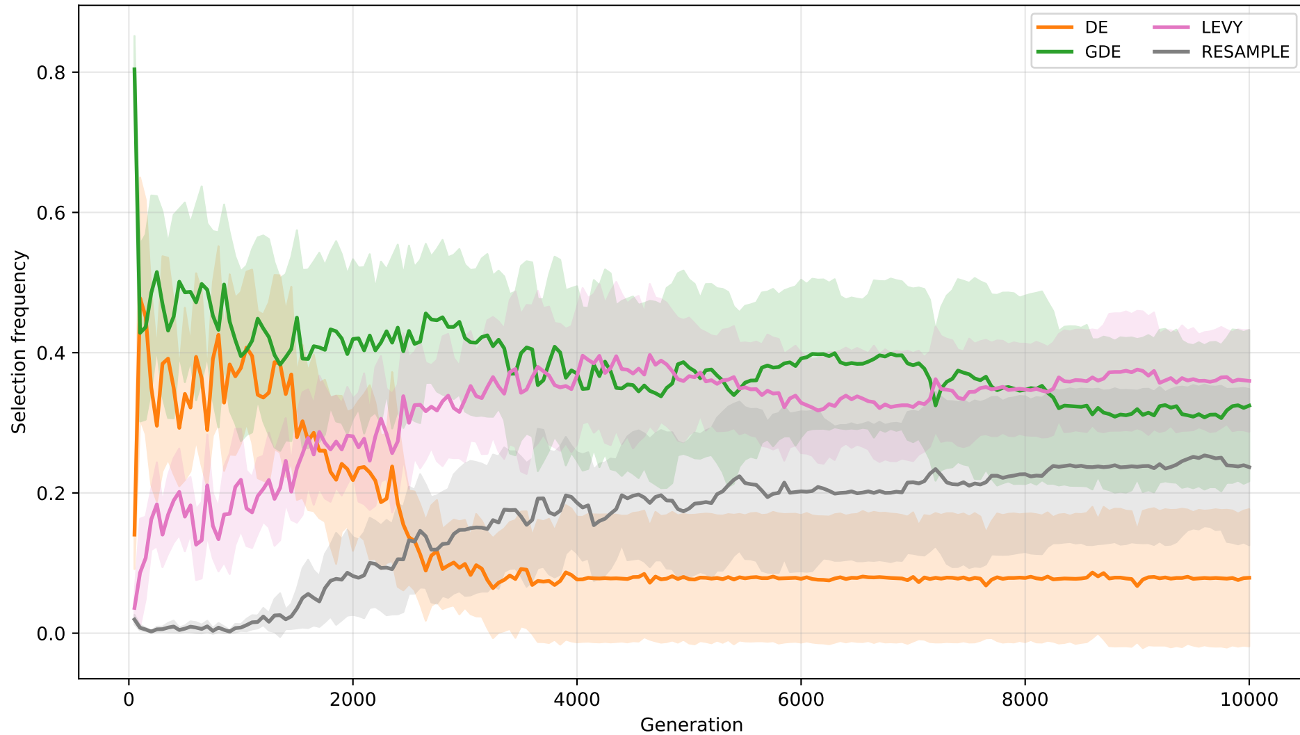
T100 Bandit Operator Frequency (dev, mean \pm 95% CI)
