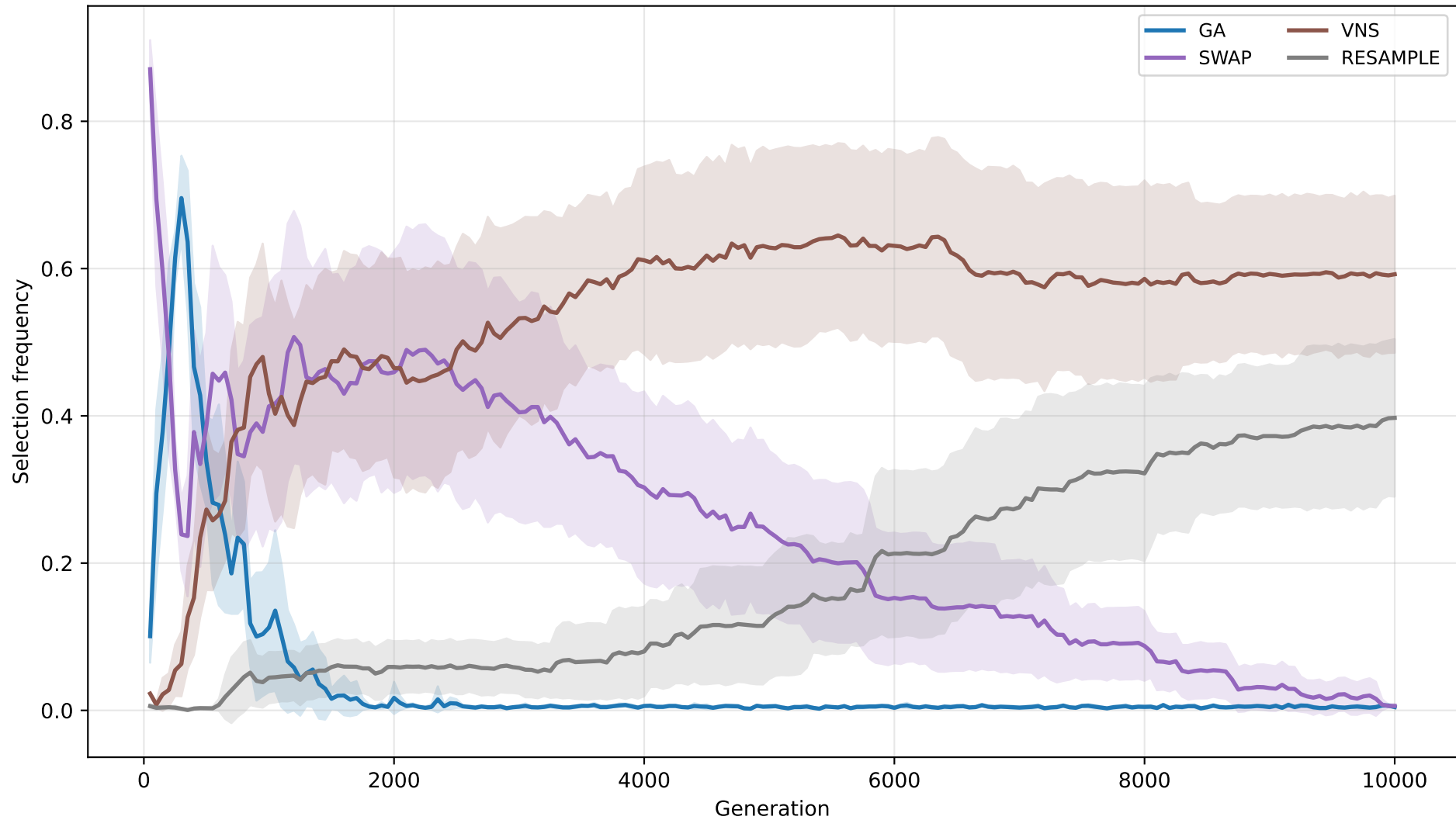
T100 Bandit Operator Frequency (seq, mean \pm 95% CI)
