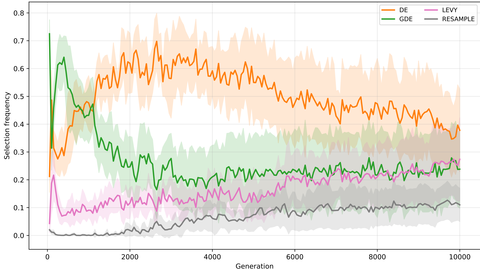
T200 Bandit Operator Frequency (dev, mean \pm 95% CI)
