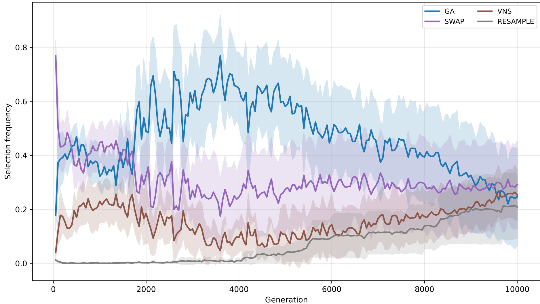
T200 Bandit Operator Frequency (seq, mean \pm 95% CI)
