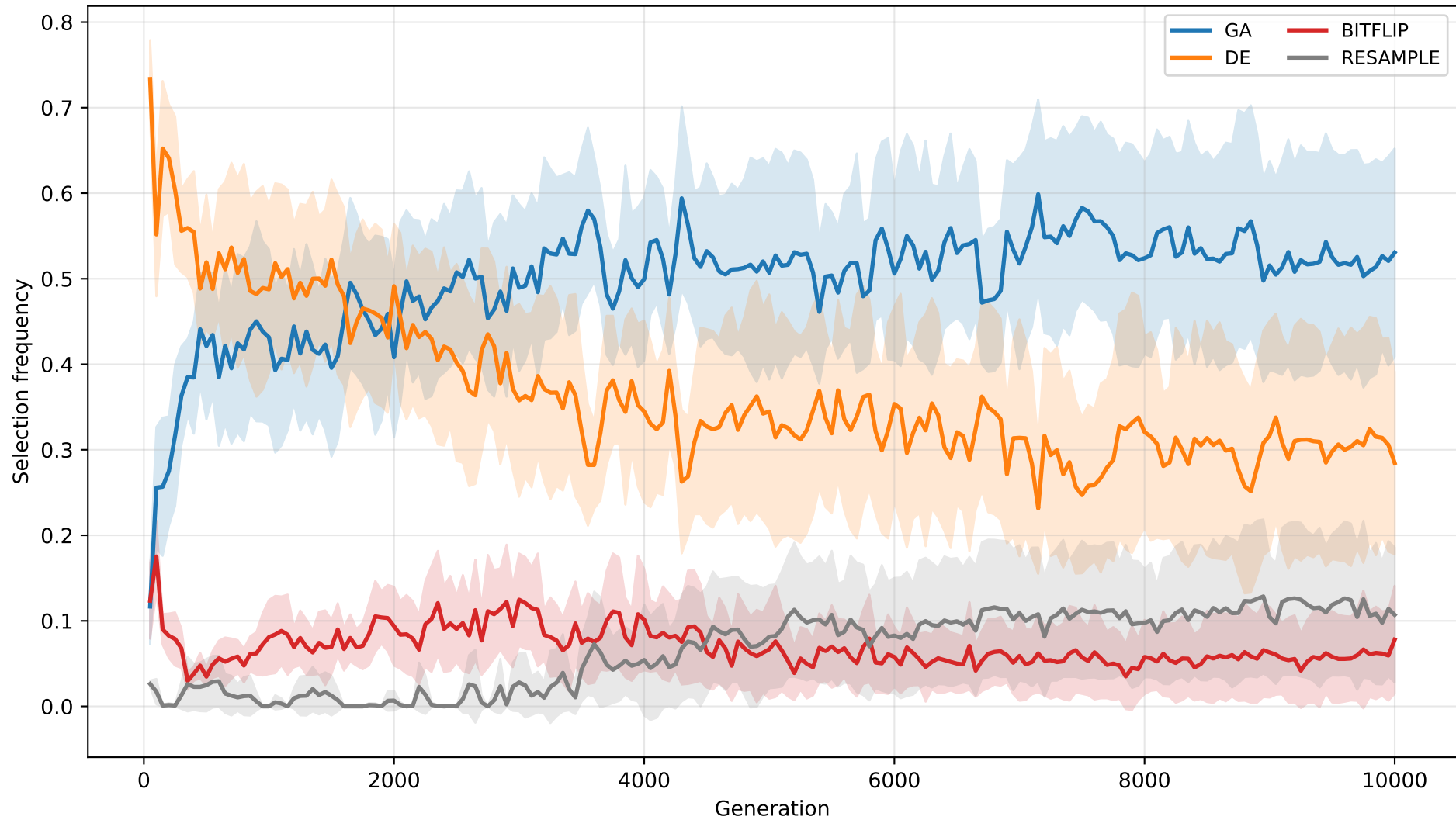
T500 Bandit Operator Frequency (offload, mean \pm 95% CI)
