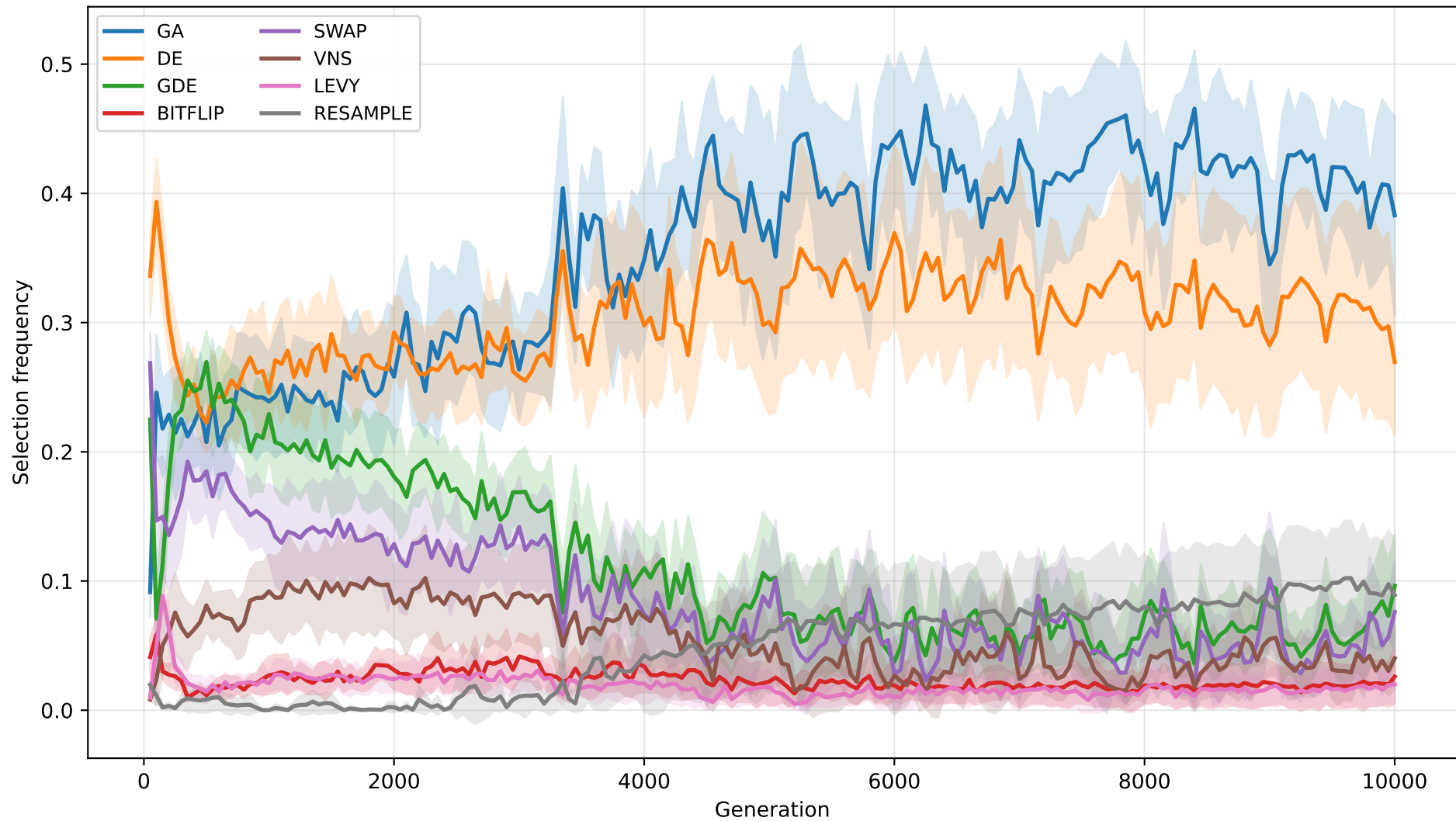
T500 Bandit Operator Frequency (overall, mean \pm 95% CI)
