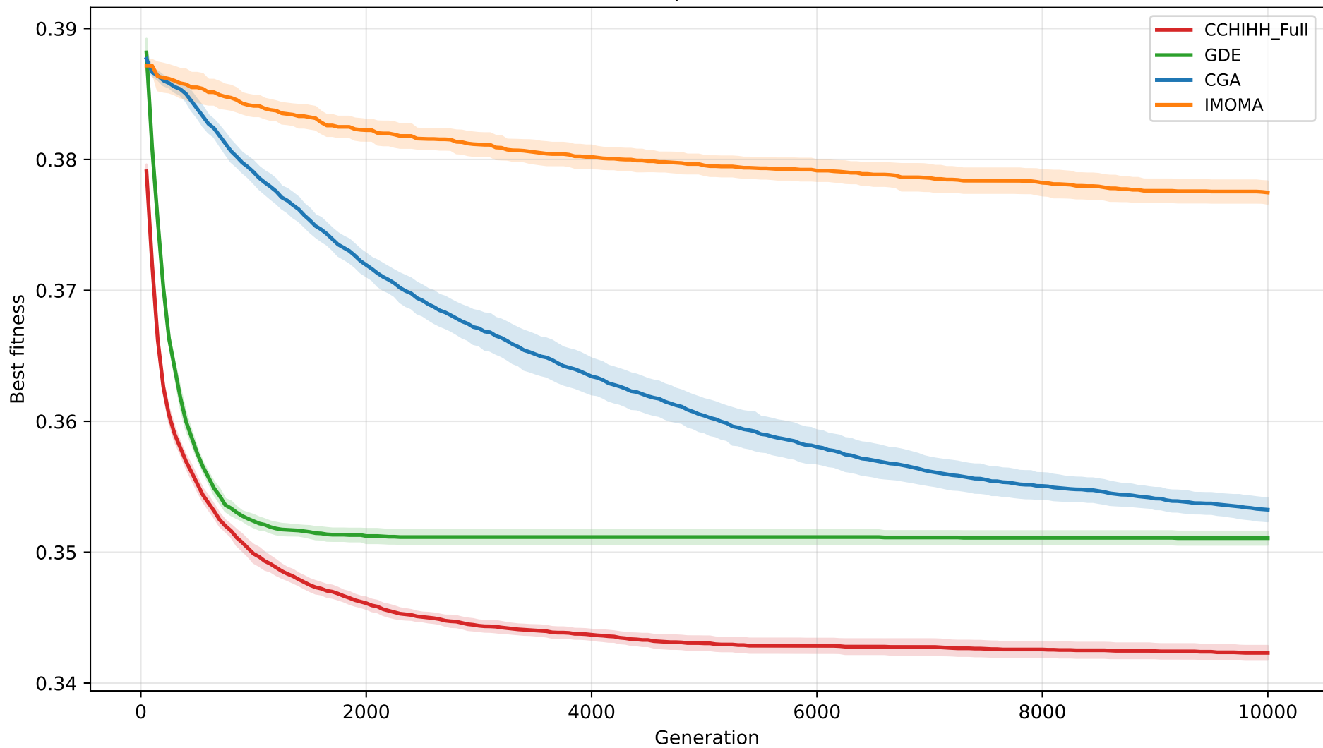
T100 Baseline Comparison (mean \pm 95% CI)
