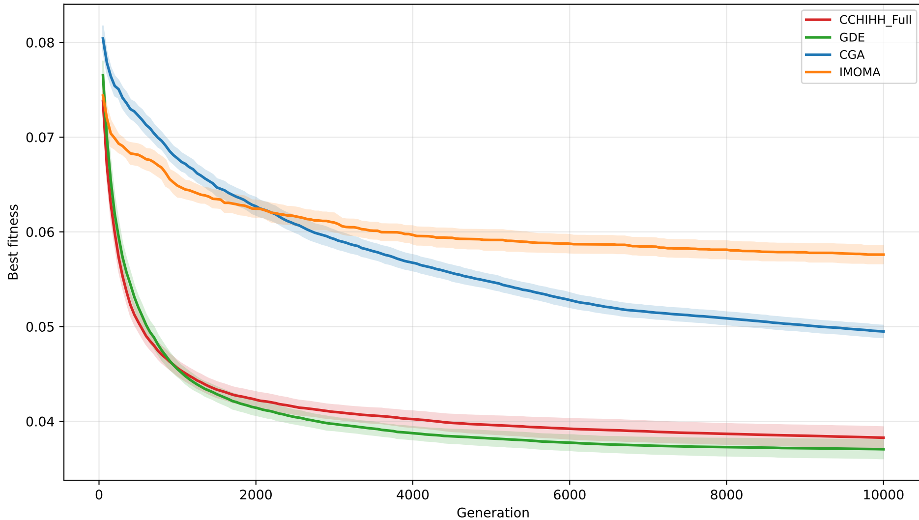
T200 Baseline Comparison (mean \pm 95% CI)
