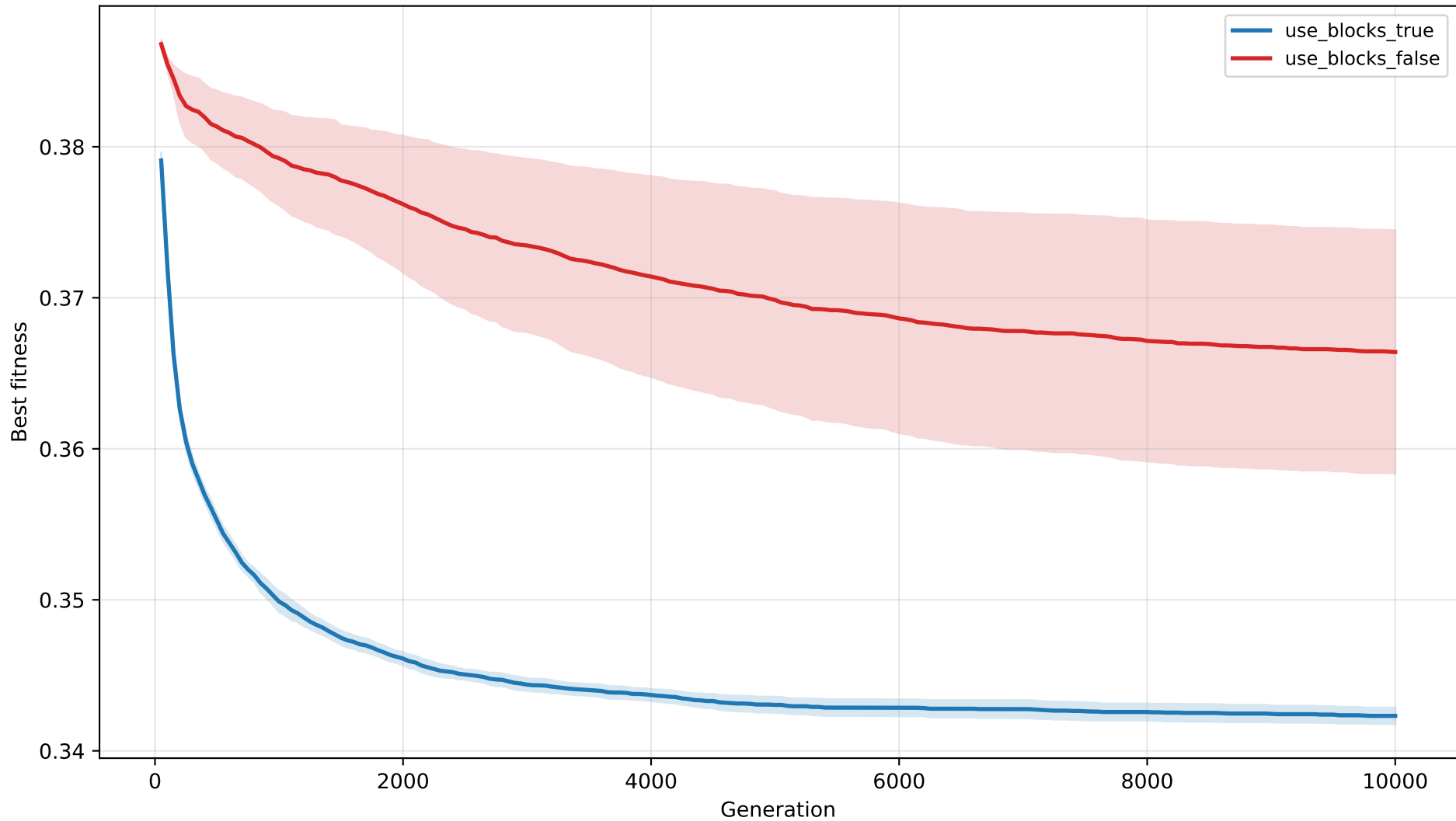
T100 Cooperative Coevolution Ablation (mean \pm 95% CI)
