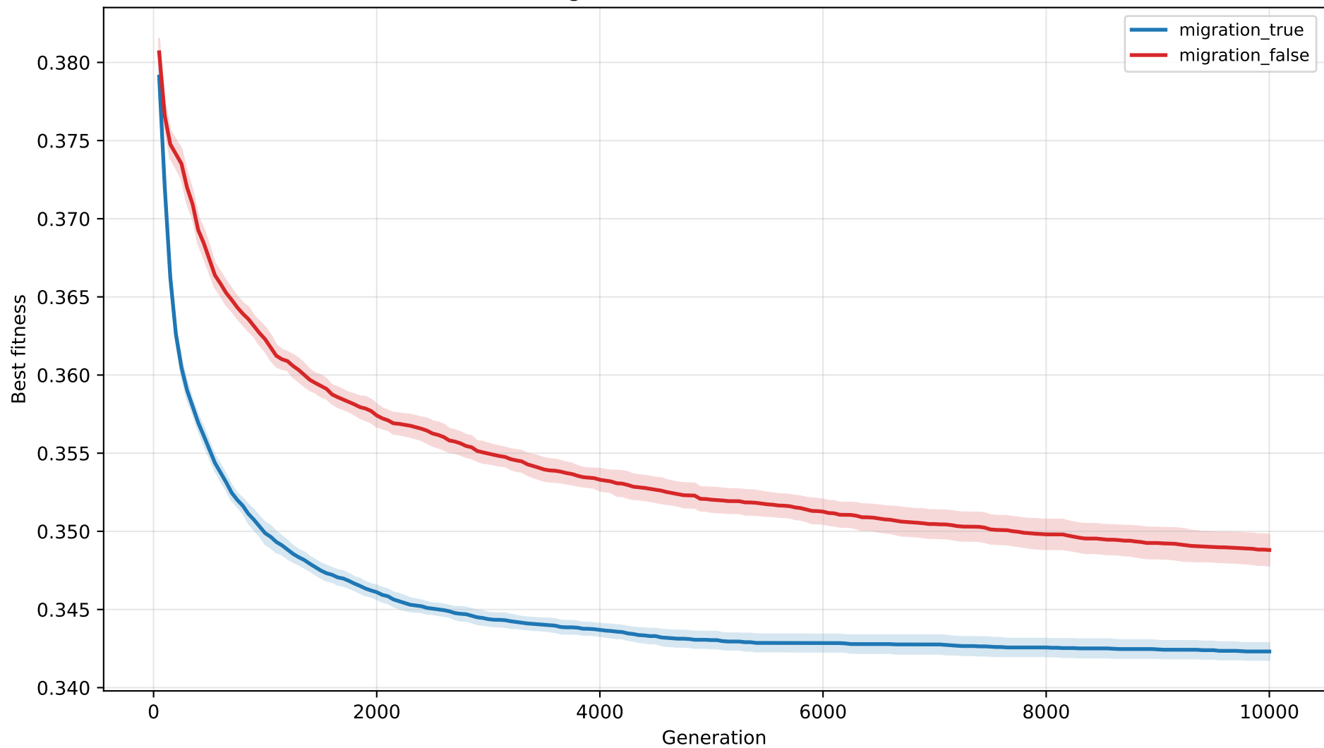
T100 Migration Ablation (mean \pm 95% CI)
