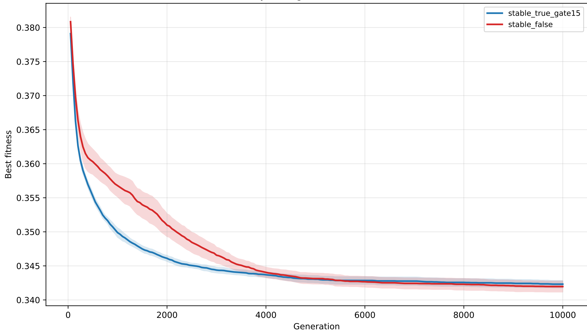
T100 Stability Gating Ablation (mean \pm 95% CI)
