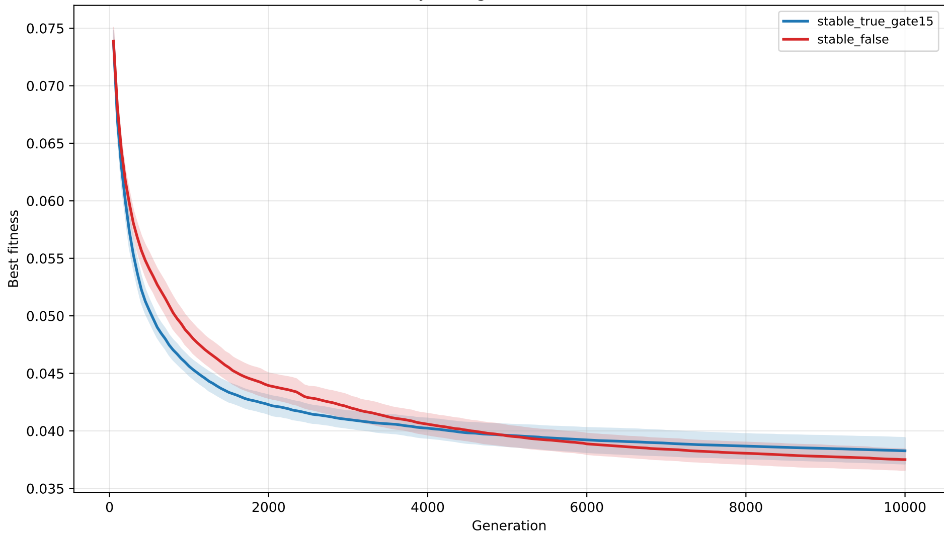
T200 Stability Gating Ablation (mean \pm 95% CI)
