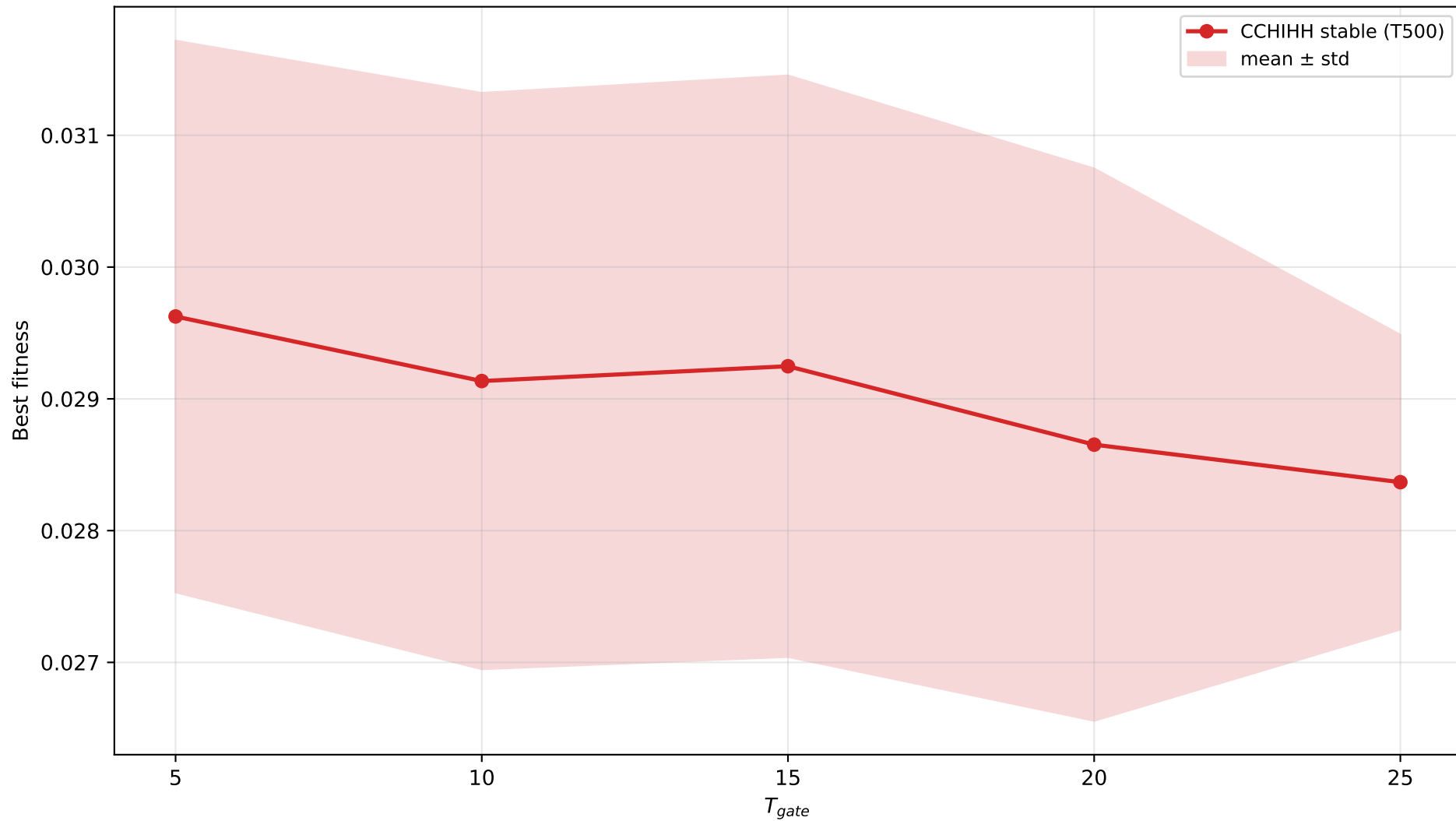
T500: Fitness vs resample gate (gen=10000)
