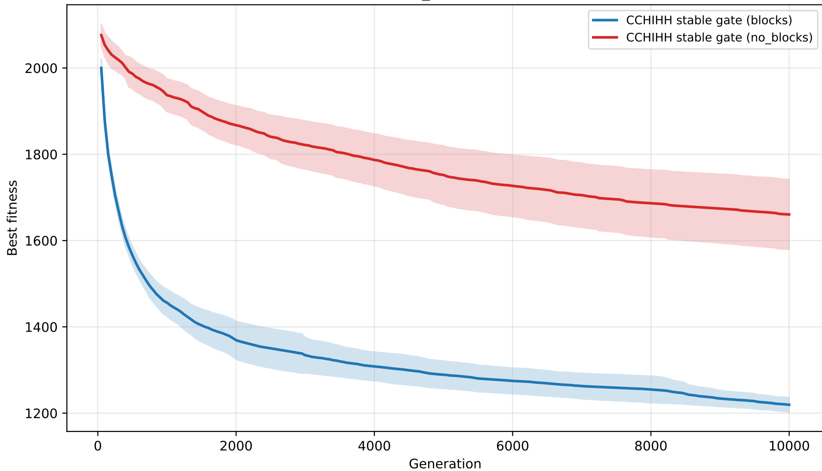
T500: blocks vs no_blocks (mean \pm 95% CI)
