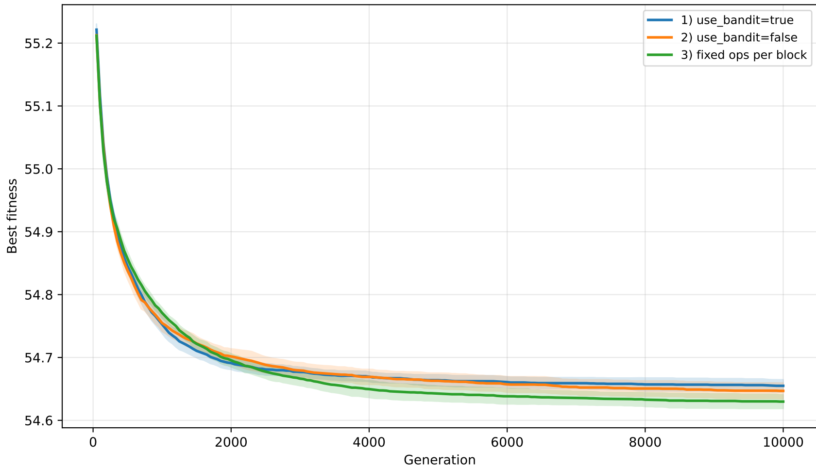
CCHIIHH Ablation: 1,2,3 (mean \pm 95% CI)
