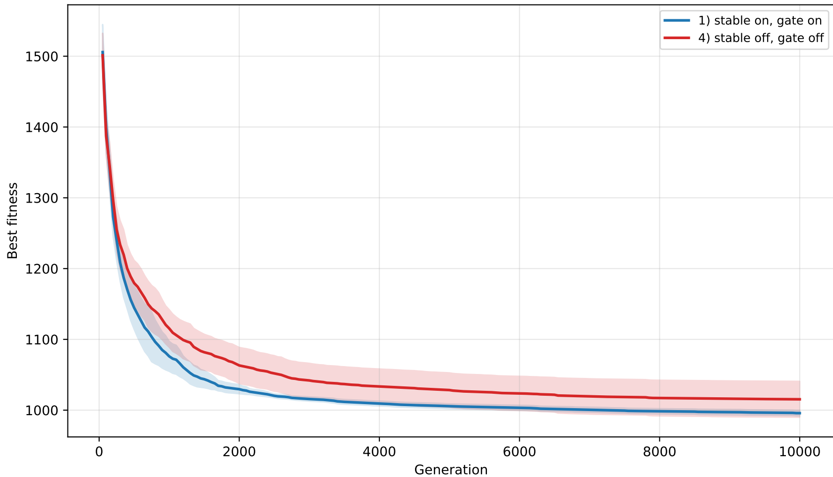
CCHIIHH Ablation: 1 vs 4 (mean \pm 95% CI)
