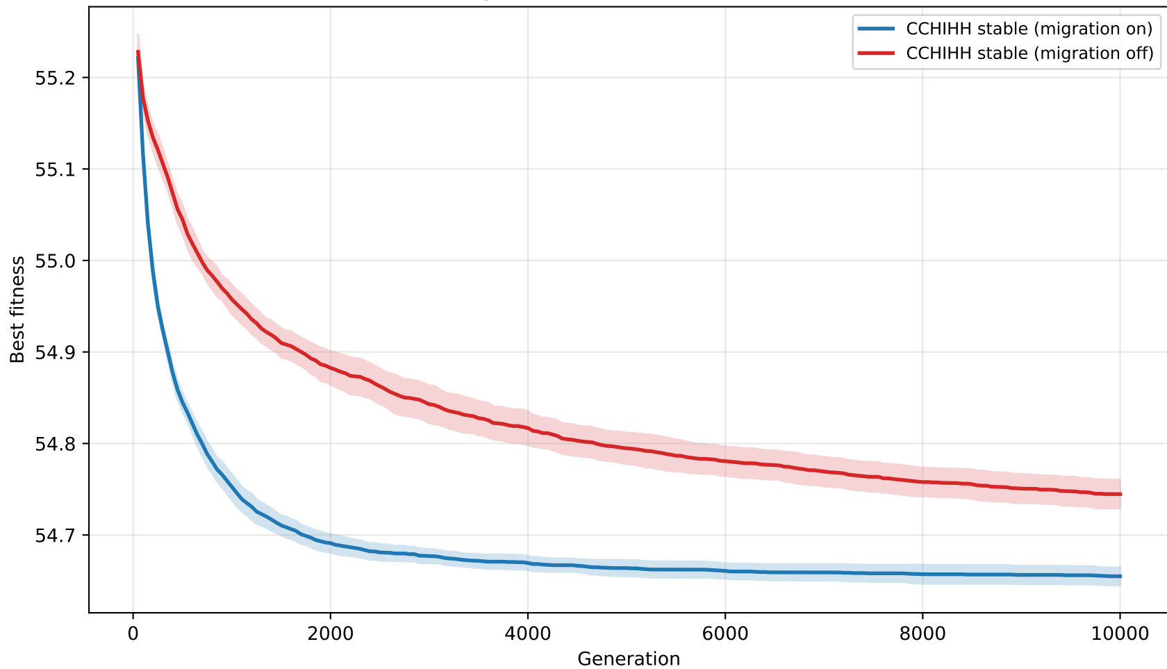
T100: migration on vs off (mean \pm 95% CI)
