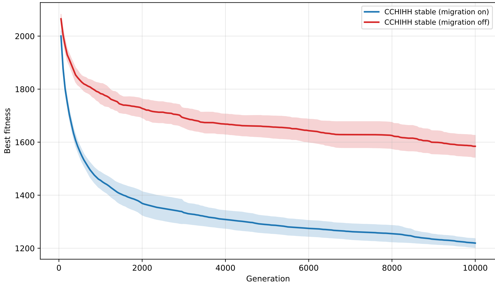
T500: migration on vs off (mean \pm 95% CI)
