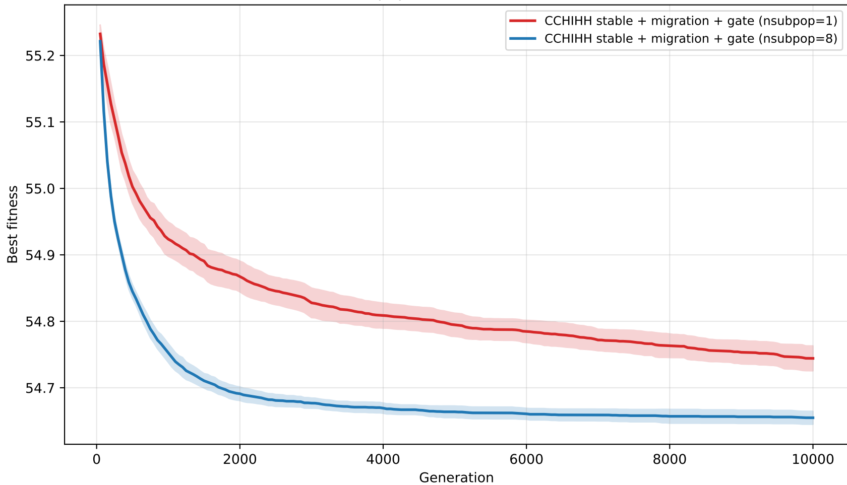
T100: nsubpop=1 vs 8 (mean \pm 95% CI)
