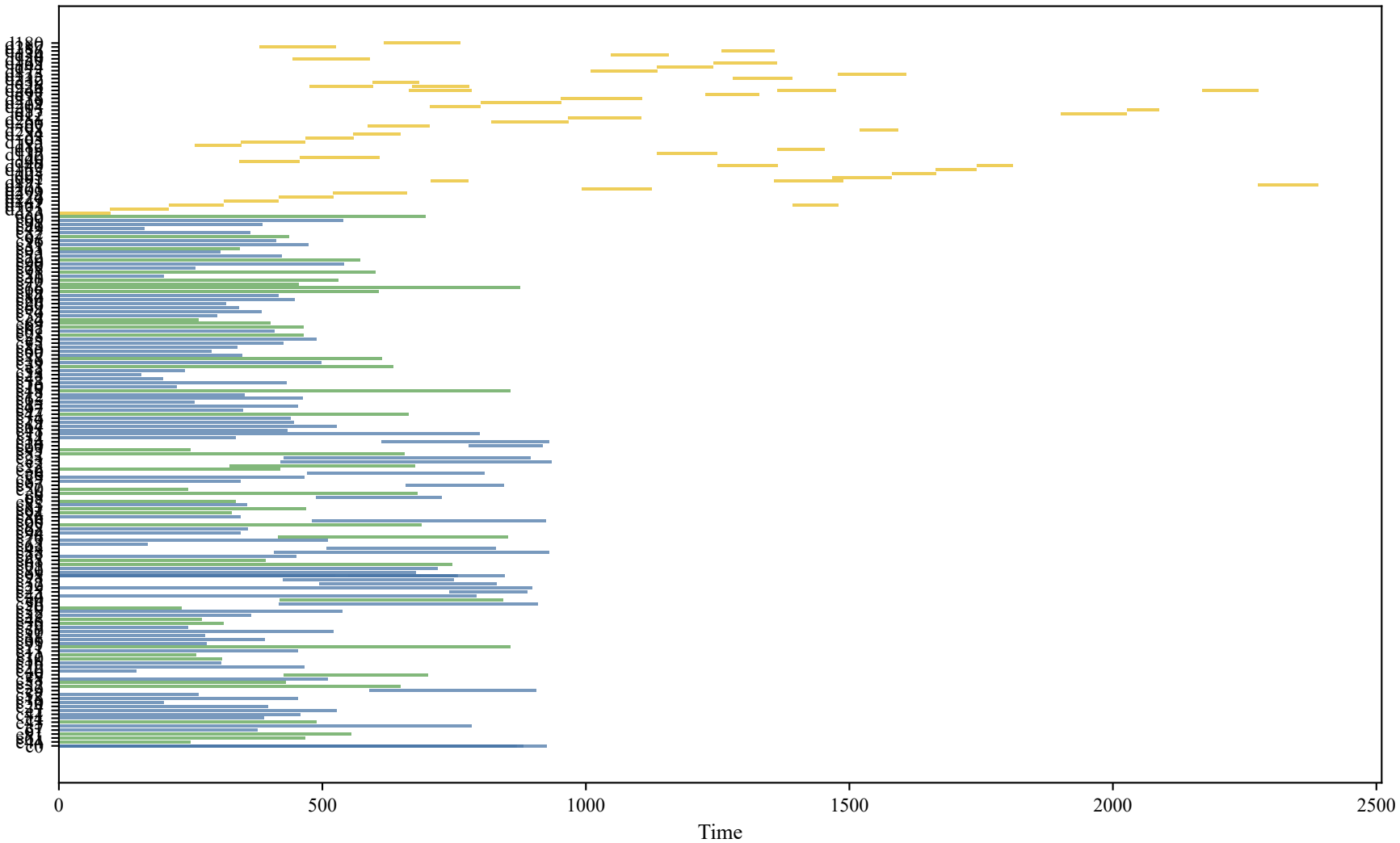
T200 best CCHIIH schedule (seed 5), makespan=934.81, energy=47.14
