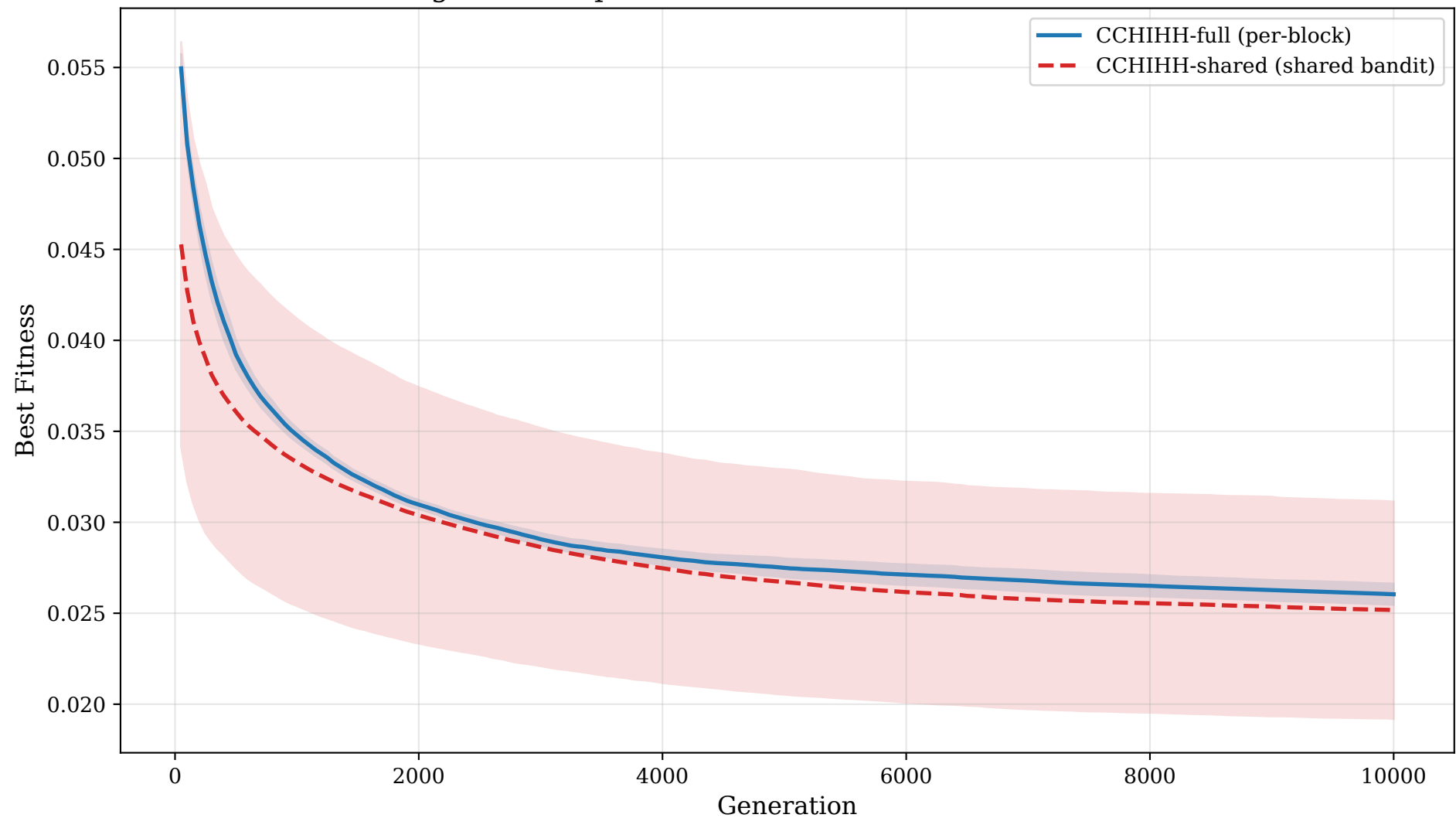
Convergence Comparison on T500: Per-block vs Shared Bandit
