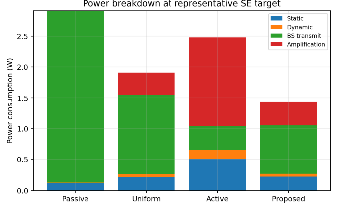
Fig. 5. Power breakdown at R_\Sigma = 12 bit/s/Hz under ES.
