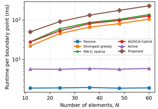
Fig. 5. Runtime per boundary point versus the number of STAR-RIS elements.
