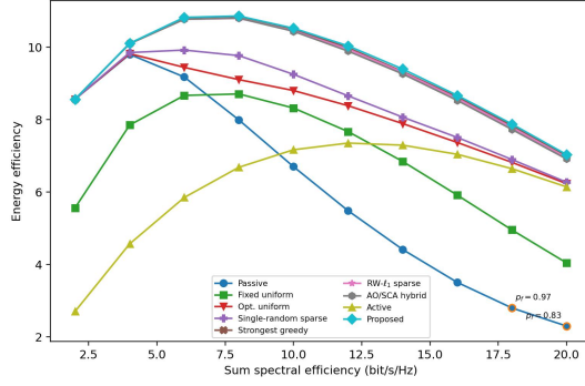
Fig. 2. Approximated EE-SE boundary.
