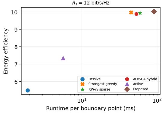
Fig. 6. EE-runtime tradeoff at R_{\Sigma} = 12 bit/s/Hz.
