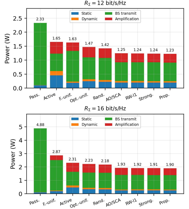
Fig. 4. Power distribution at R_\Sigma = 12 and 16 bit/s/Hz, sorted by total power.
