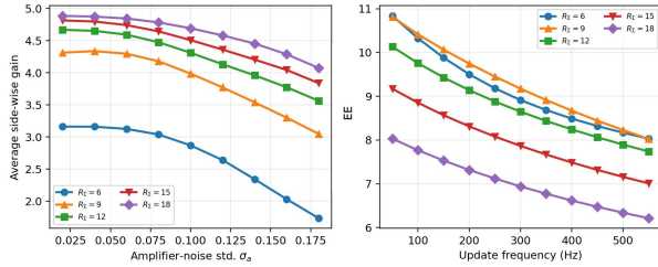
Fig. 3. Hardware sensitivity versus amplifier noise and switching overhead.
