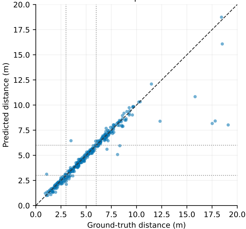
MoGe + MLP calibration MAE 0.334 m | Bias -0.197 m
