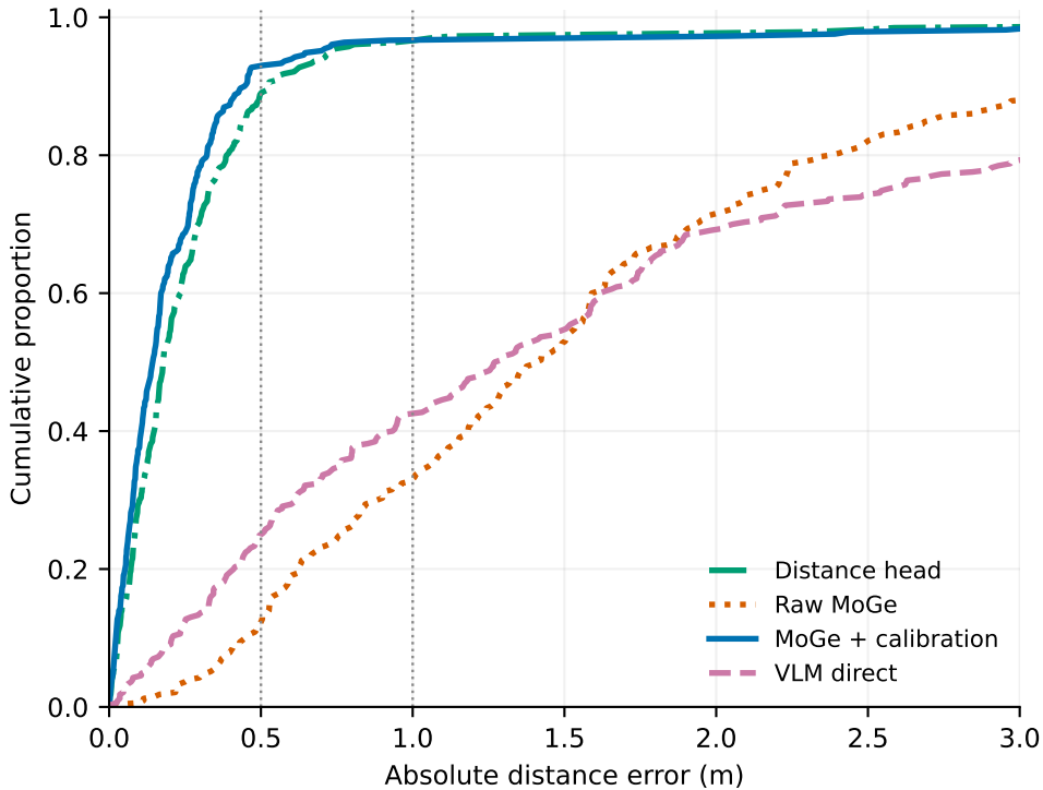
Absolute-error distribution (n=330)
