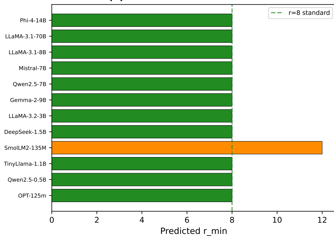
(b) LoRA Rank Recommendation
