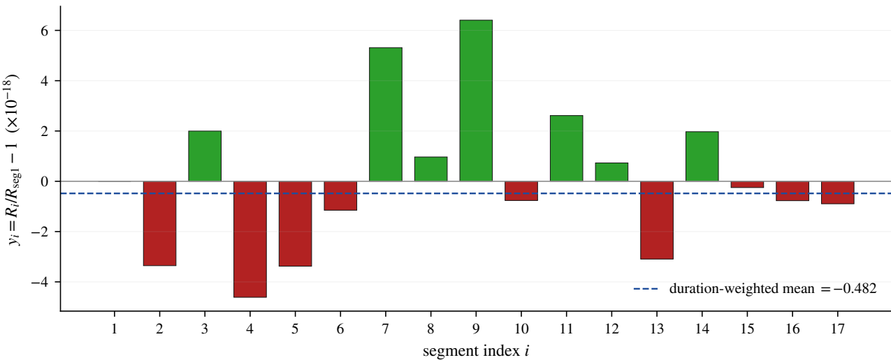
(a) Per-segment Yb/Sr clock-ratio deviation
