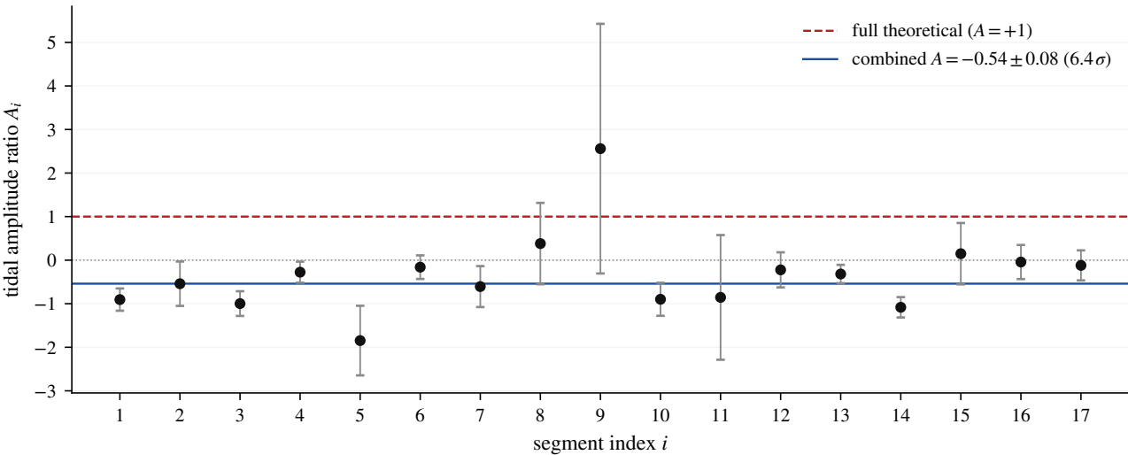
(b) Per-segment tidal-redshift amplitude (1200-s triangular fit)
