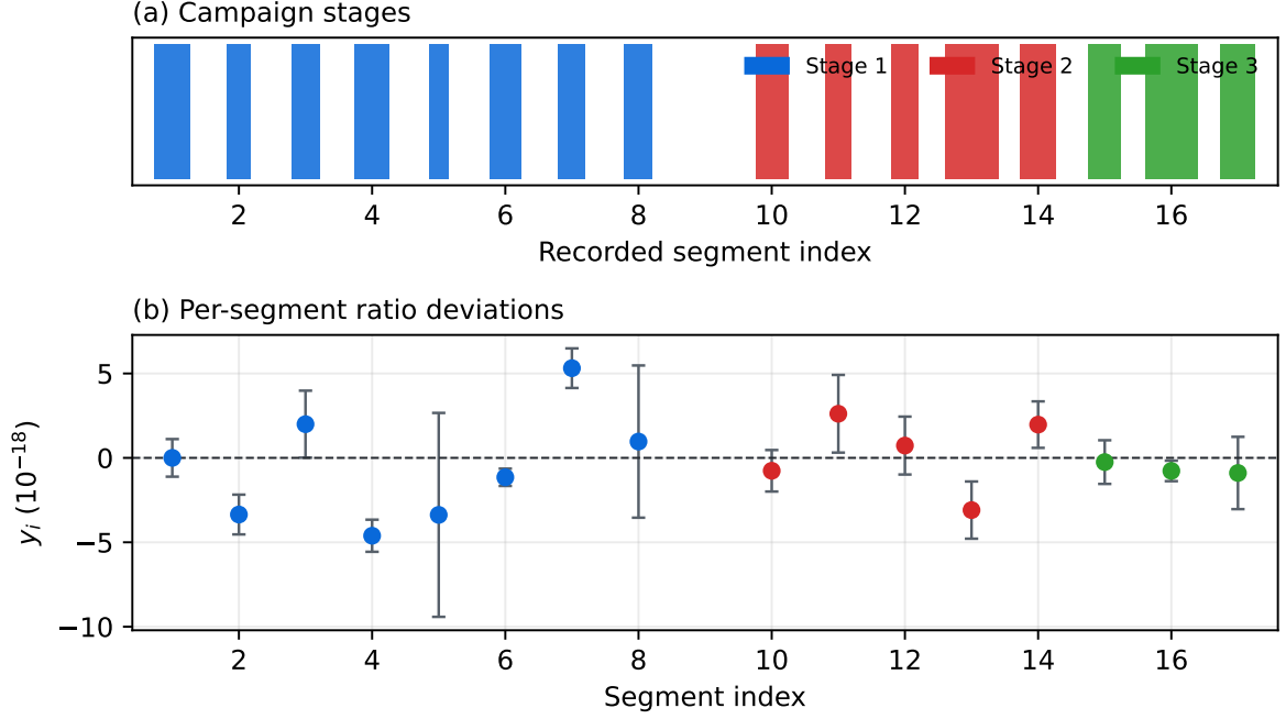
Figure 2: Campaign and per-segment data. (a) Recorded segments coloured by measurement stage; bar widths scale with the square root of the retained sample count. (b) Per-segment ratio deviations y_i with their statistical uncertainties; the dashed line marks zero deviation.
