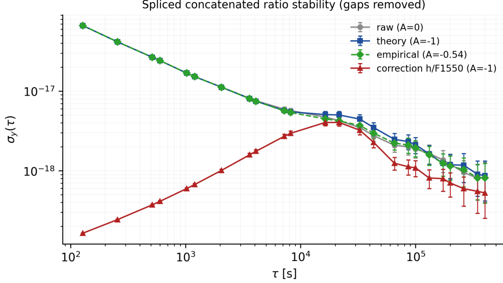
Figure 6: Spliced concatenated stability. Overlapping Allan deviation \sigma_y(\tau) of the seventeen segments placed end-to-end on one continuous 1s record (aligned pure-data span 11.7 d, gaps removed; \tau up to 4.63 d), for the raw ( A = 0 ), theory ( A = -1 ) and empirical ( A = -0.54 ) scenarios, with the correction-term curve and Riley–Howe EDF error bars.
