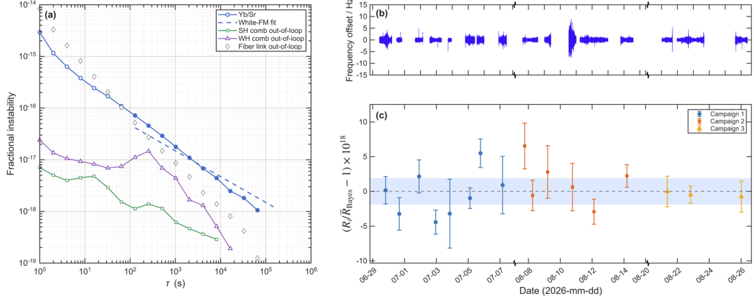
Figure 2: Clock-ratio data. The segment stability and the 17–16 per-segment Yb/Sr ratios R_i ( segment 9 excluded ) give the deviation y_i = R_i/R_{\text{seg1}} - 1 whose duration-weighted mean is -0.482 \times 10^{-18} -0.639 \times 10^{-18} and whose segment-to-segment scatter is \sigma(y_i) = 2.98 \times 10^{-18} \sigma(y_i) = 2.58 \times 10^{-18} .
