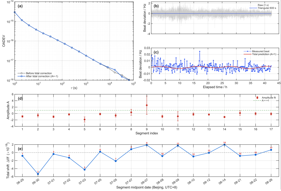
Figure 3: Tidal influence and its correlation. The tidal modulation of the comparison frequency is resolved at 6.4σ across the 17 segments (combined 1200-s-window fit gives a historical amplitude A = -0.54 \pm 0.08 , at estimate near A = -0.54 (about half the theoretical magnitude), and at ; overlapping-window significance is not interpreted as a detection statistic. At the segment- mean level the ratio deviation y_i is positively correlated with the tidal shift \Delta f/f (Pearson r = +0.518 r = +0.429 ).
