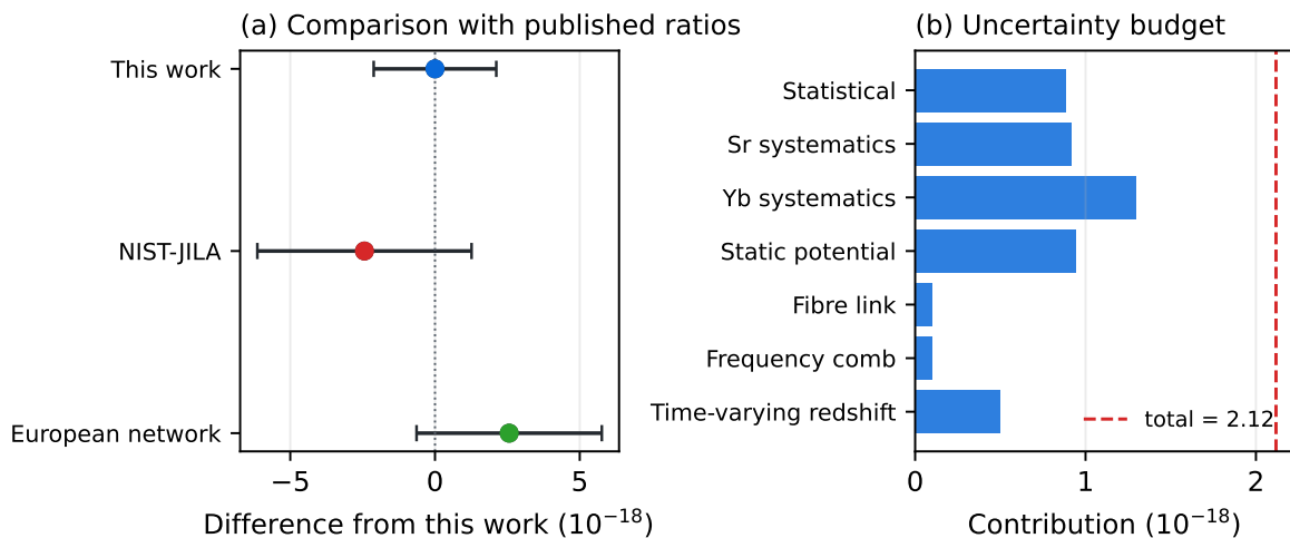
Figure 3: Comparison and budget. (a) Differences between this work and the published Yb/Sr ratios, with their quoted uncertainties. (b) Components of the total standard uncertainty; the dashed line marks the quadrature total.
