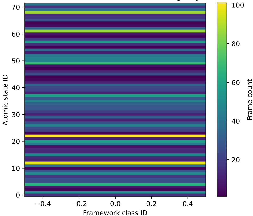
Atomic-state/framework-class contingency
