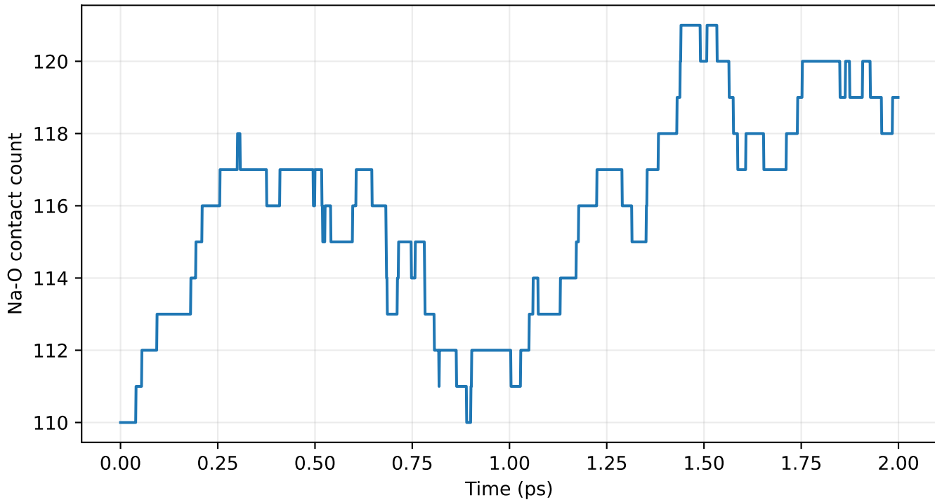
Na-O contact-count time series
