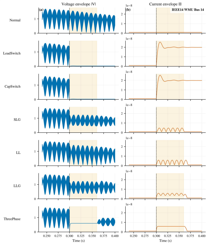
(a) IEEE14
