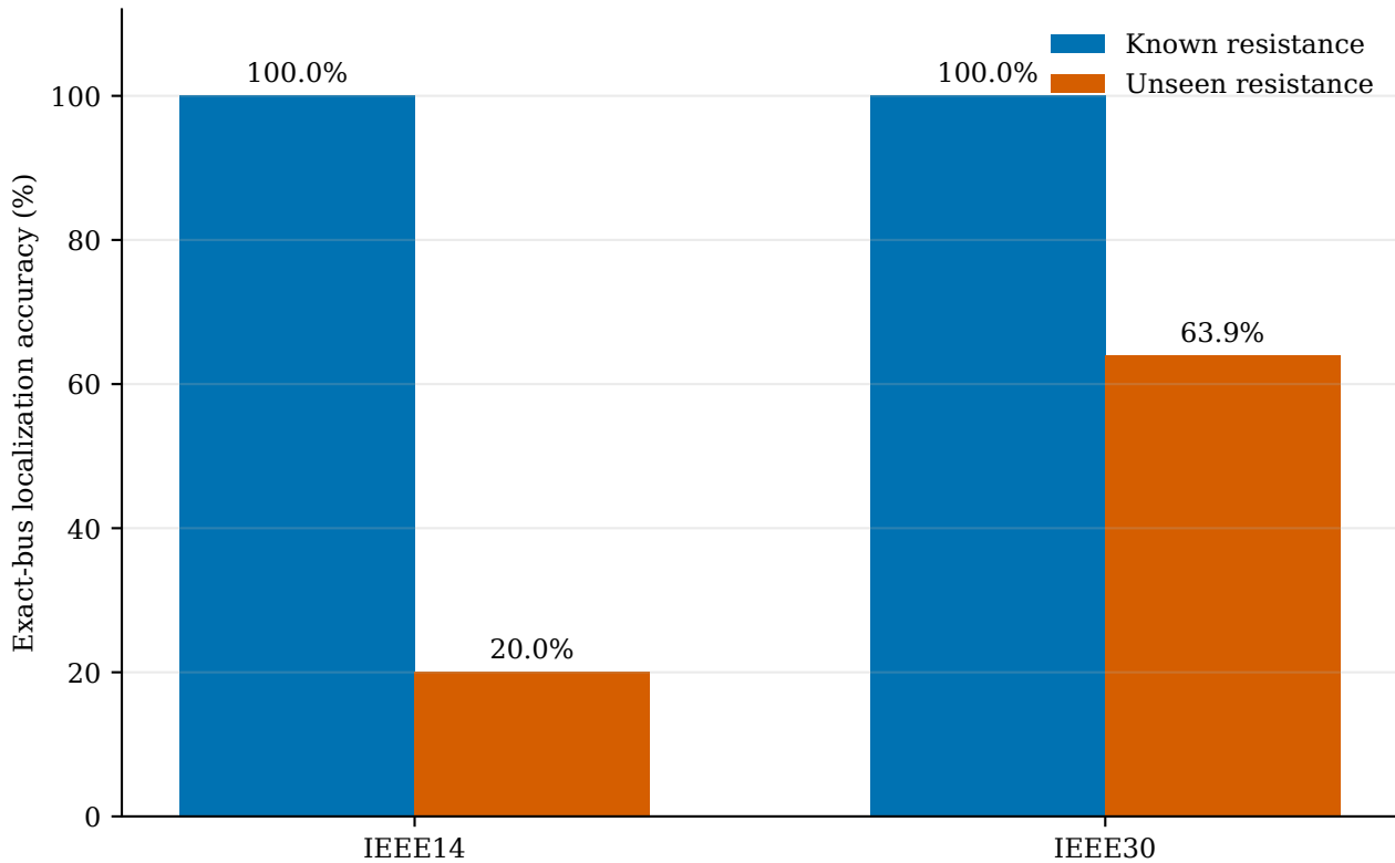
Performance degradation under unseen fault resistance
